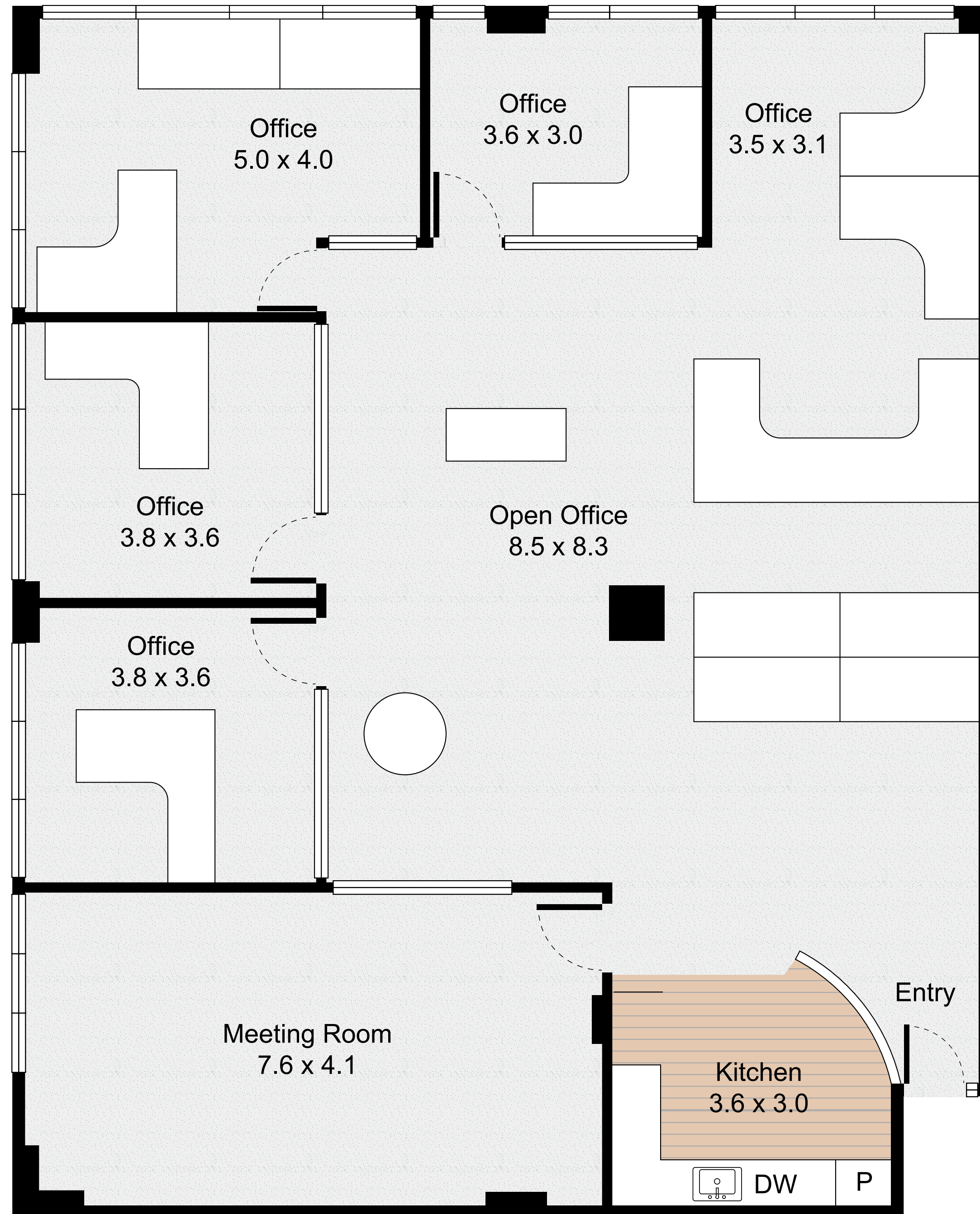
FLOOR PLAN
