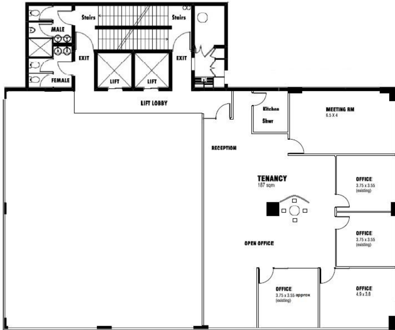
Tenancy Layout Plan Not to Scale
